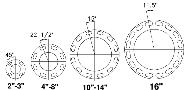
Flange Orientation
